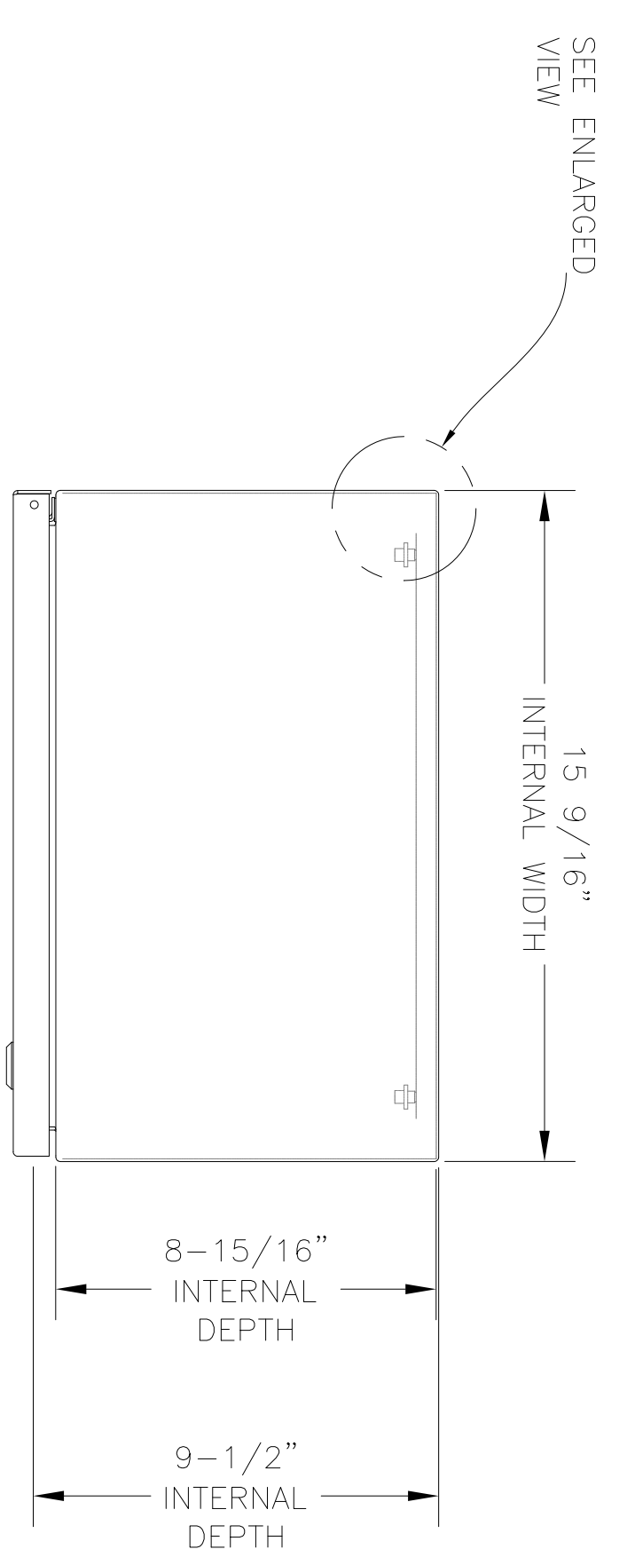
TOP VIEW YUCO ENCLOSURE 20"X16"X10" SINGLE DOOR NEMA 4 SCALE: FULL
