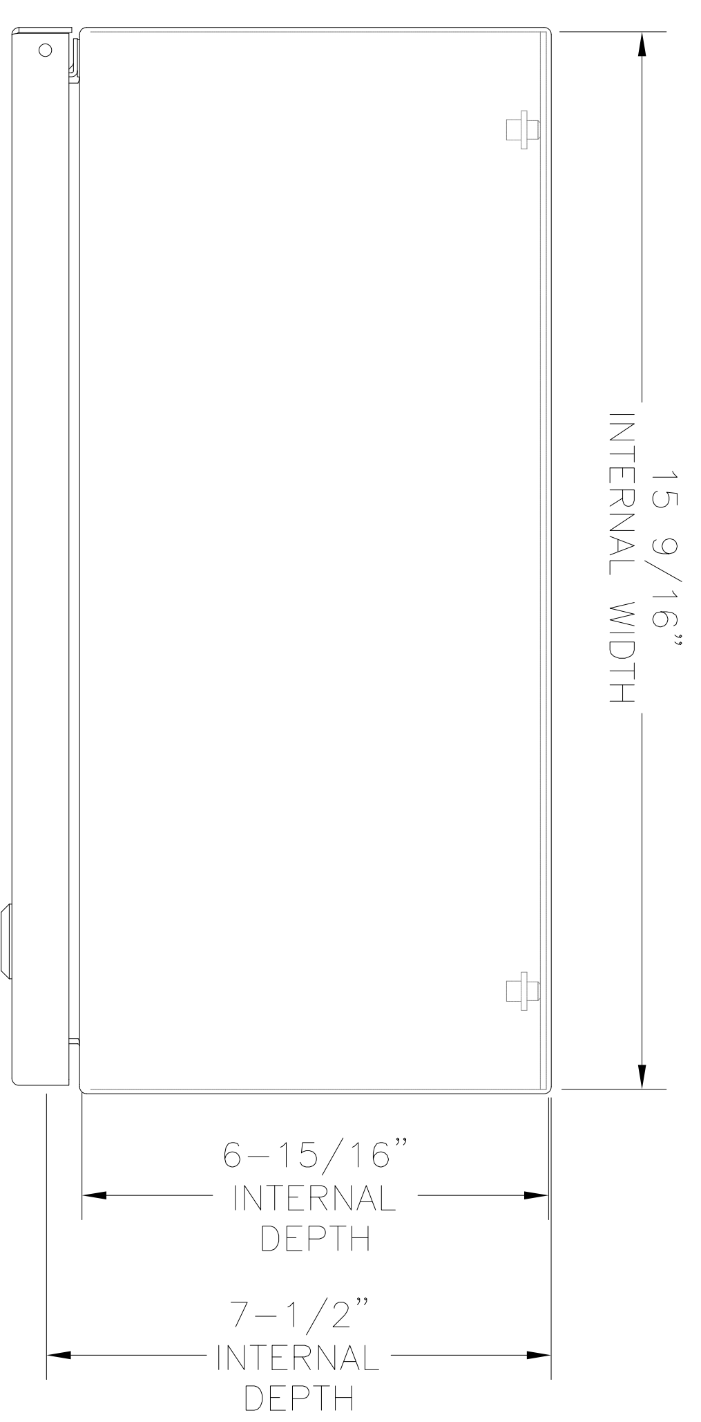
TOP VIEW YUCO ENCLOSURE 16"X16"X8" SINGLE DOOR NEMA 4 SCALE: 1:1
