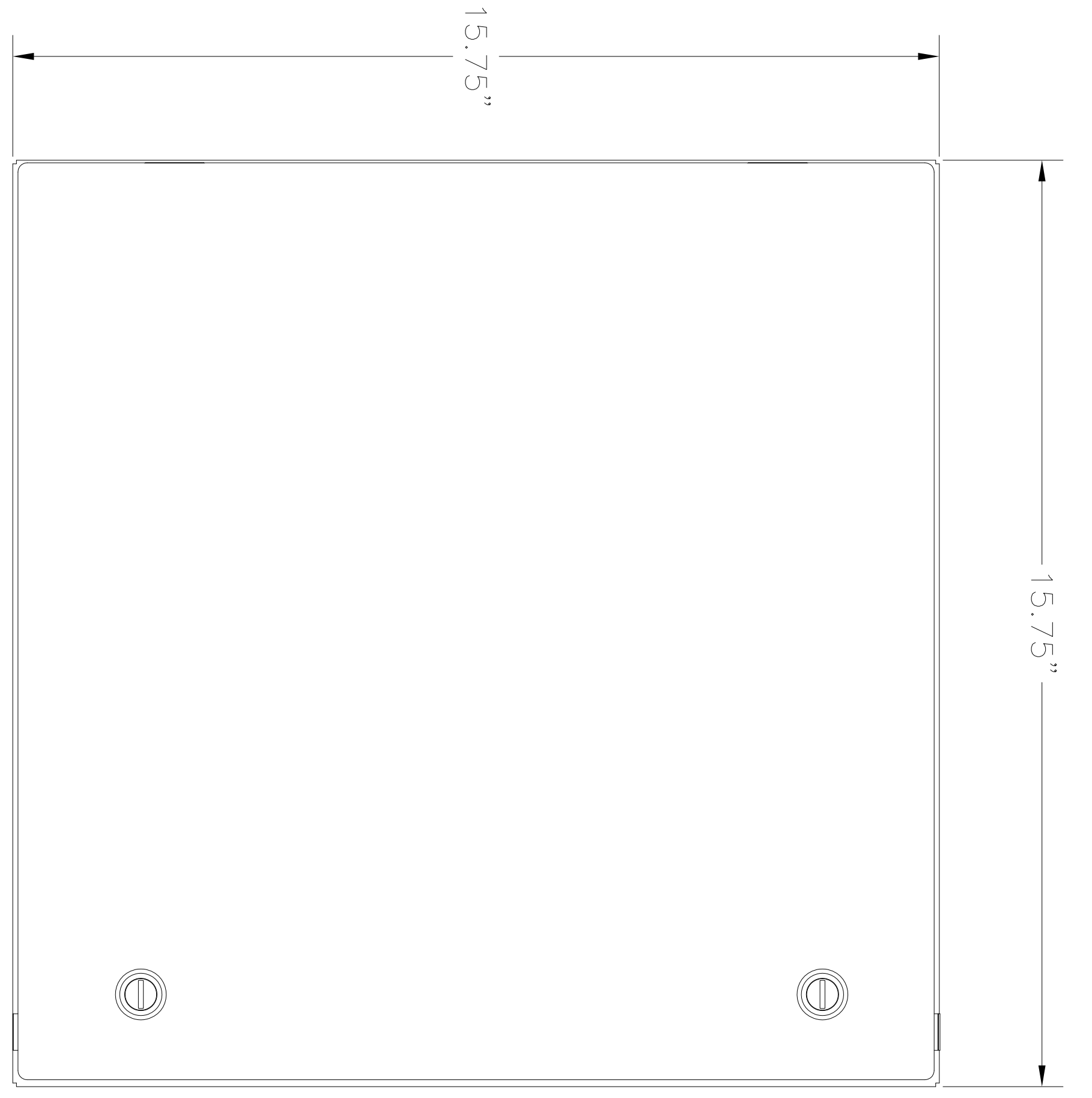
TOP VIEW YUCO ENCLOSURE 16"X16"X8" SINGLE DOOR NEMA 4 SCALE: 1:1
